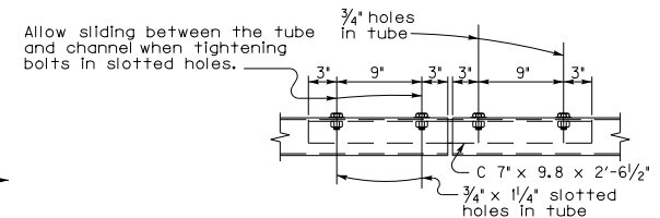
OPEN JOINT
