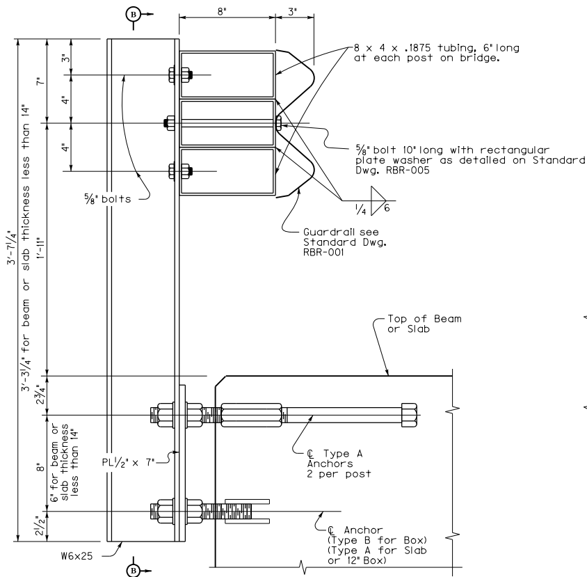
TYPICAL SECTION
