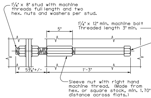
TYPE A ANCHOR DETAIL
