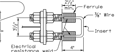
TYPE B ANCHOR DETAIL
